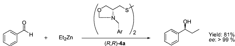
Scheme 1. The enantioselective addition of diethylzinc to benzaldehyde using the disulfide ( R,R )- 4a
