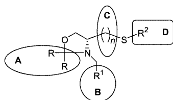
Figure 1. General combinatorial approach to the synthesis of sulfur-oxazolidine ligands with the variables R and n ( A–D )
