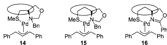
Figure 2. The bite angle effect
