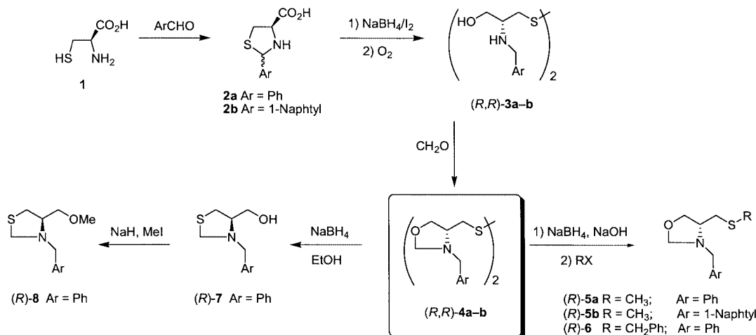
Scheme 2. Synthesis of sulfur-oxazolidine ligands by the general combinatorial approach
