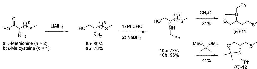
Scheme 3. Synthesis of ligands with variations in R or n (A and C, Figure 1)
