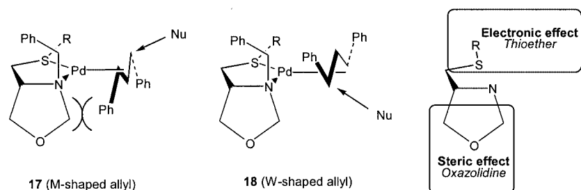
Figure 3. Diastereomeric (allyl)palladium complexes; enantioselectivity as a result of steric and electronic effects
